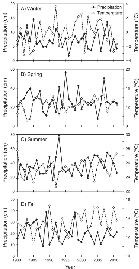
FIG. 3. Trends in precipitation (solid diamonds and line) and temperature (open diamonds and dashed line) over the study period for (A) winter, (B) spring, (C) summer, and (D) fall.
