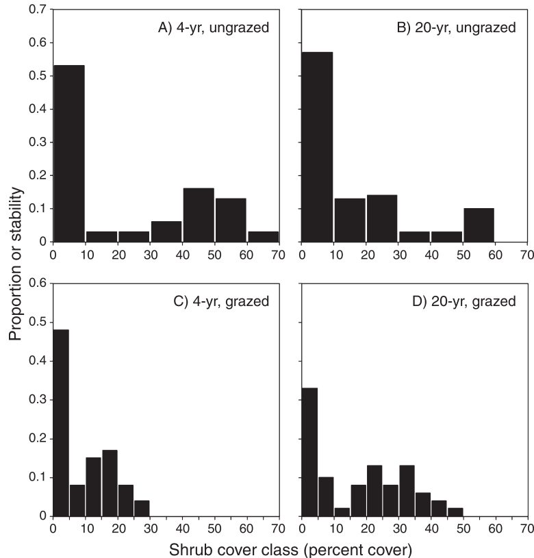
FIG. 5. Histograms of shrub cover in ungrazed (A) 4-yr and (B) 20-yr treatments, and in grazed (C) 4-yr and (D) 20-yr treatments. AIC values for the three distributions are (A) unimodal 373, bimodal 330, Johnson SI 339; (B) unimodal 392, bimodal 378, Johnson SI 392; (C) unimodal 274, bimodal 248, Johnson SI 250; and (D) unimodal 257, bimodal 225, Johnson SI -1025.
