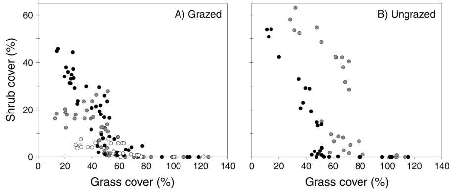
FIG. 4. Relationship between grass cover and shrub cover in (A) grazed and (B) ungrazed treatments. Fire treatment symbols are as in Fig. 2. In grazed treatments, the 4-yr-fire treatment has linear AIC/r^2 of 344/0.45; logistic AIC/r^2 of 325/0.63. The 20-yr-fire treatment has linear AIC/r^2 of 348/0.64; logistic AIC/r^2 of 319/0.82. In the ungrazed treatments, the 4-yr-fire treatment has linear AIC/r^2 of 257/0.49; logistic AIC/r^2 of 257/0.53. The 20-yr-fire treatment has linear AIC/r^2 of 239/0.56; logistic AIC/r^2 of 200/0.90.
