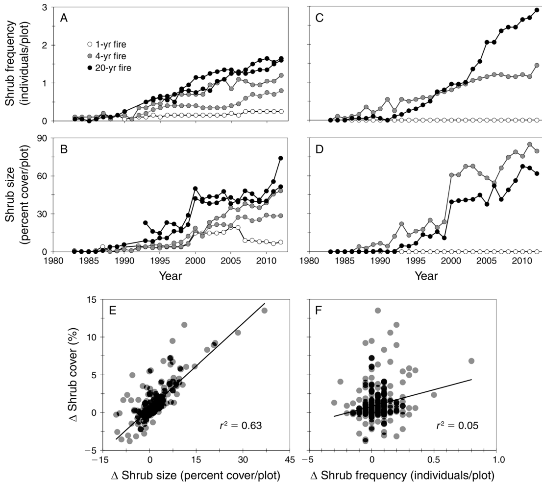
FIG. 6. The trends in (A and C) shrub frequency and (B and D) shrub size index in (A and B) grazed and (C and D) ungrazed treatments. Also shown is (E) the relationship between year-to-year changes in shrub size index and shrub cover, and (F) the relationship between year-to-year changes in shrub frequency and shrub cover. For panels (E) and (F), all treatments are shown together because relationships were similar across treatments.
