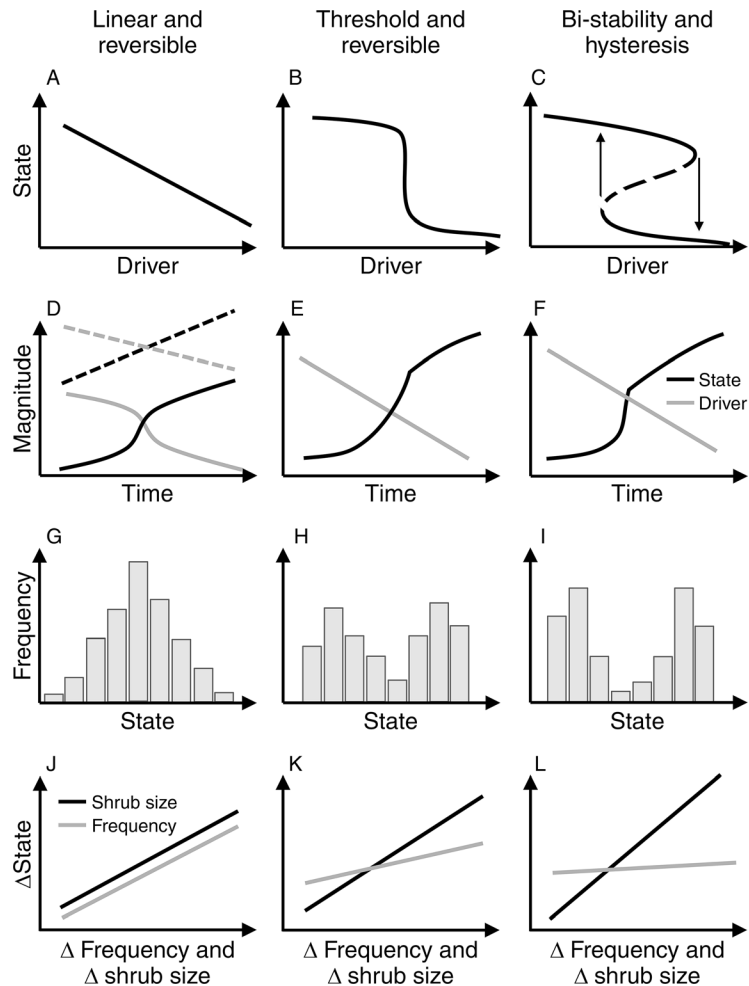
FIG. 1. Depiction of different types of (A–C) internal dynamics in ecosystems with varying linearity and hysteresis and (D–I) the expected behavior. Panels (J–L) depict hypotheses specific to our study system, linking positive feedback mechanisms to threshold transitions. The first row shows the relationship between state and driver variables in (A) linear, (B) threshold, and (C) alternative attractor systems (systems manifesting bi-stability and hysteresis). For panels (A–C), black lines depict stable equilibria, dashed lines are unstable “repellers,” and arrows depict a regime shift between alternative attractors. Here, we use shrub cover as the proposed state variable (i.e., a slow changing variable) and we explore potential driver variables. Panels (D–F) show the expected temporal behavior of an ecosystem’s state (black line) in the three different system types, under different scenarios of changes in driver variables over time (gray lines). Note that in panel (D), dotted lines show how a system with linear internal dynamics should respond to an abrupt shift in the driver variable. Panels (G–I) show the expected frequency (no. shrubs/plot) diagrams for the different system types. Panels (J–L) depict our hypothesis that shrub expansion in our study system should be correlated with increases in shrub size because this type of expansion is related to positive feedback mechanisms ( \Delta stands for “change in”). Panels (A–I) are based on Holling (1973), Noy-Meir (1975), May (1977), Walker (1981), Folke et al. (2004), Scheffer et al. (2004), Schroder et al. (2005), and Bestelmeyer et al. (2011), while panels (J–L) are based on concepts developed in Ratajczak et al. (2011), D’Odorico et al. (2012), and Nippert et al. (2013)
