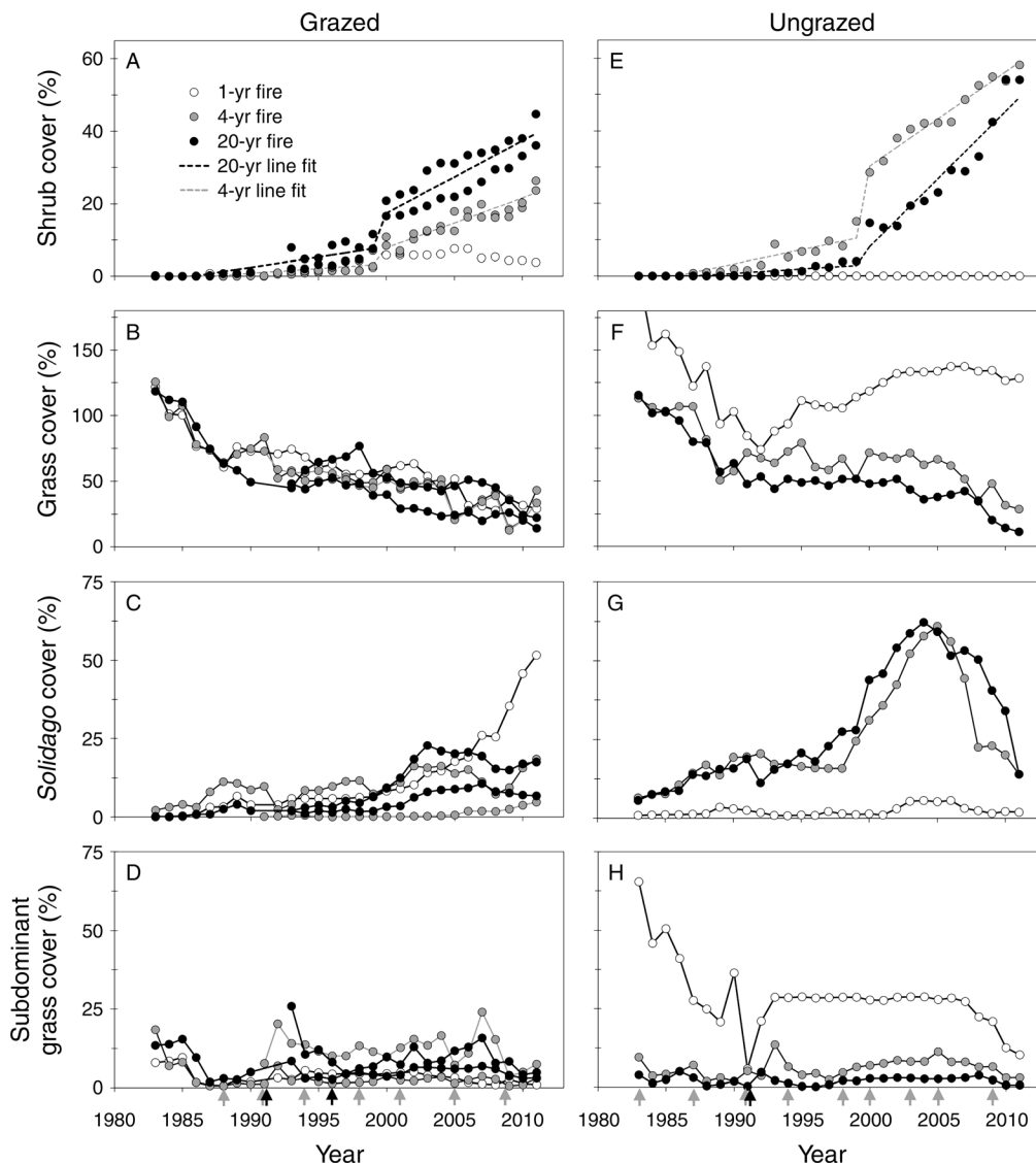
FIG. 2. Temporal patterns of (A, E) shrub cover, (B, F) dominant C_4 grass cover, (C, G) Solidago spp. cover, and (D, H) subdominant grass cover, for grazed (left column) and ungrazed treatments (right column). The 20-yr-between-fires (20-yr fire) treatments appear as black circles, 4-yr-between-fires (4-yr fire) treatments as gray circles, and 1-yr-between-fires (1-yr fire) treatments as open circles. In panels (A) and (E), dashed lines show split linear fits for treatments with fire frequency >1 -yr-fire (black for 20-yr fire and gray for 4-yr fire). Arrows below panels (D) and (H) demark the timing of prescribed fires in 4-yr (gray arrows) and 20-yr fire treatments (black arrows). Note that there are two replicates for the 4- and 20-yr grazed treatments because data from slope transects was available for almost the entirety of the experiment.
